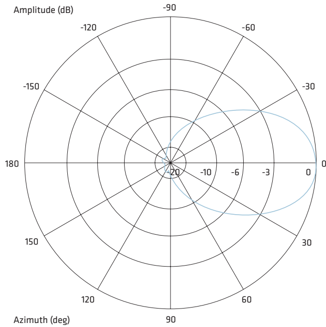
— Horizontal-Plane: Copolar
